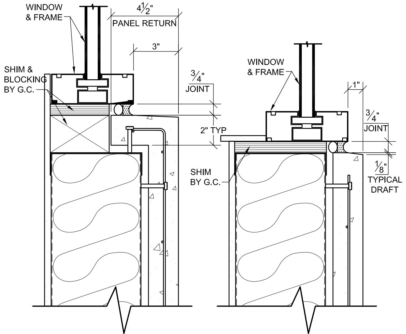
OPTIONAL WINDOW RETURN DETAIL
